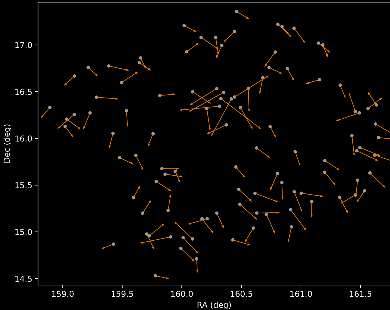
APOGEE DR17 Cluster 2 Proper Motion Vectors (n=101)
