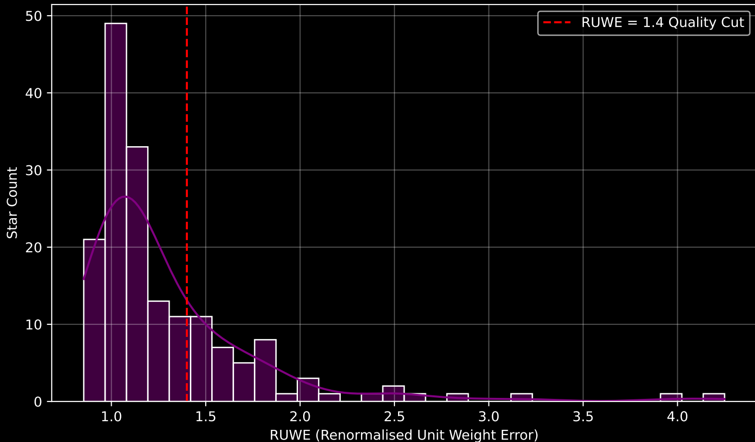
GAPOGEE DR17 Field [K2_C4_175-27_btx] RUWE Distribution (n= 171)
