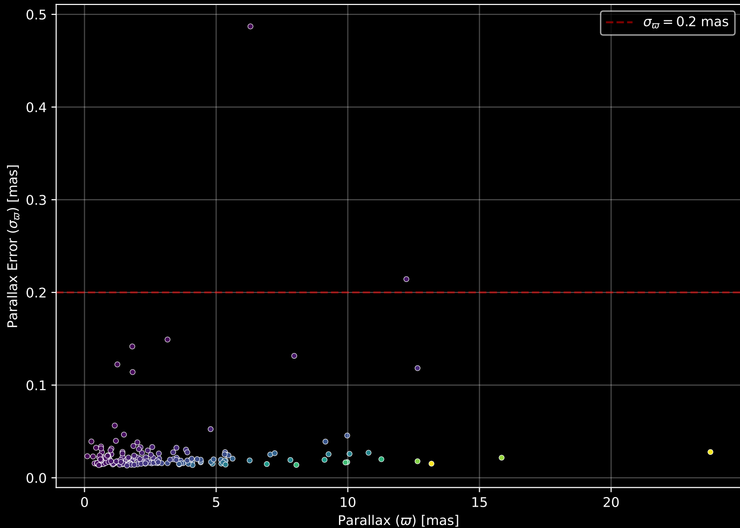
APOGEE DR17 Field: [K2_C4_175-27_btx] Parallax Quality (n= 178)
