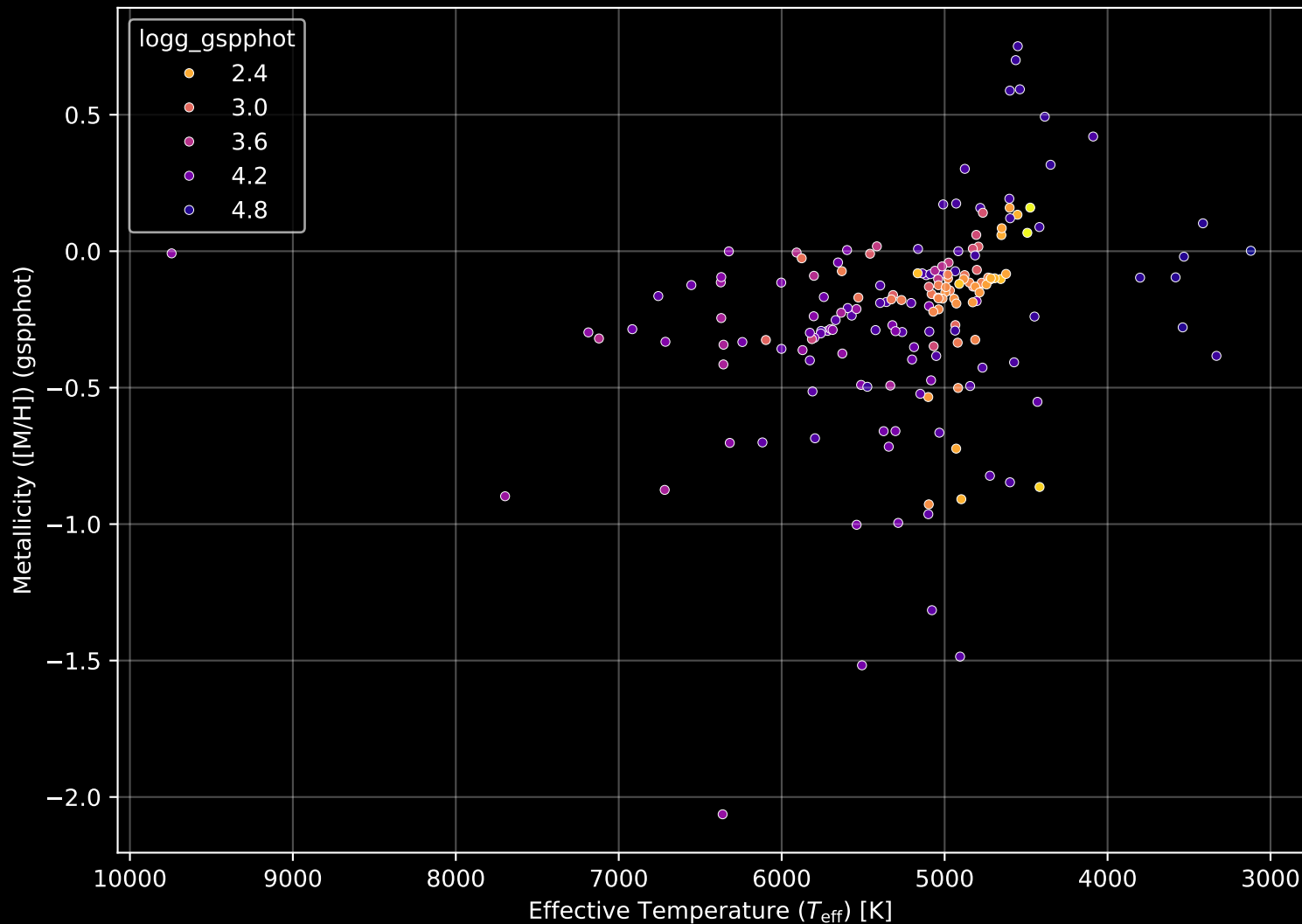
APOGEE DR17 Field: [K2_C4_175-27_btx] Stellar Population Parameters (n= 178)
