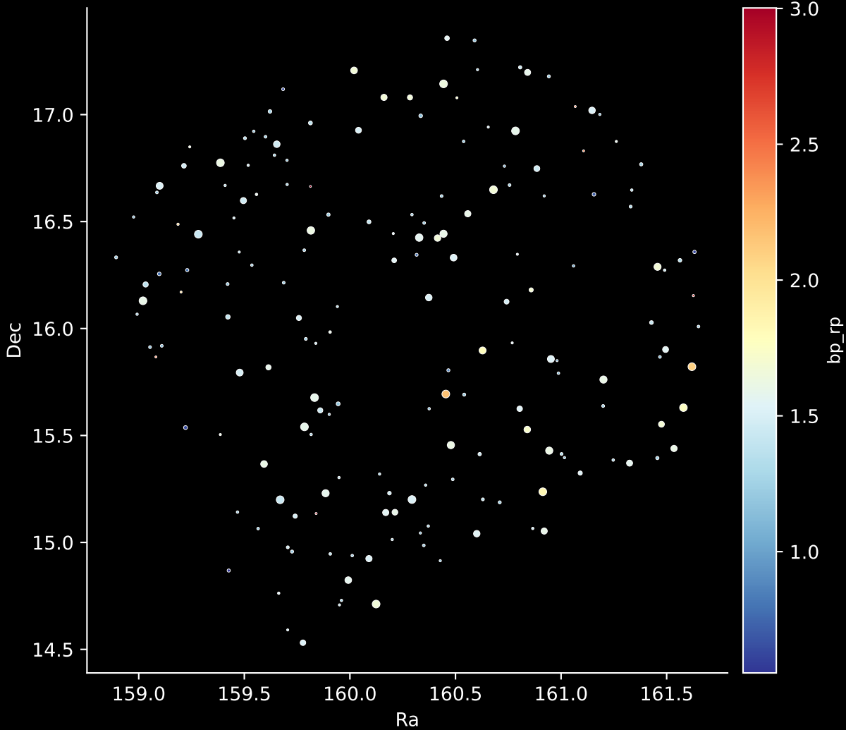
APOGEE DR17 Field: [K2_C4_175-27_btx] Stars: 178
