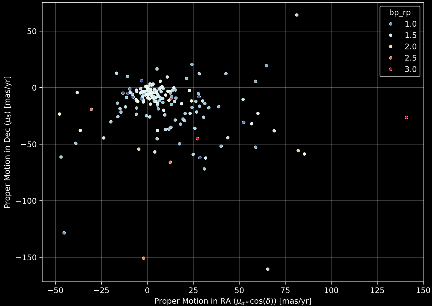
APOGEE DR17 Field: [K2_C4_175-27_btx] Proper Motion Diagram (n= 178)
