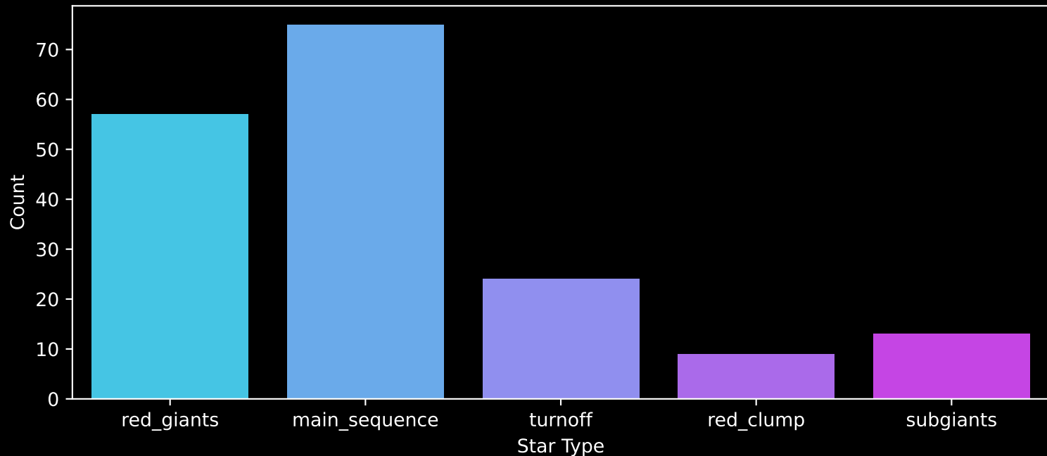
APOGEE DR17 Field: [K2_C4_175-27_btx] Count plot of Star Type
